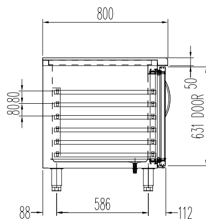
NO UPSTAND WORKTOP
