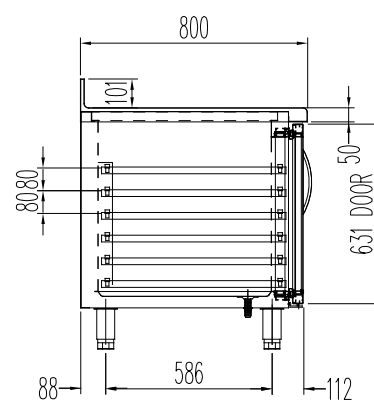
WORKTOP WITH UPSTAND
