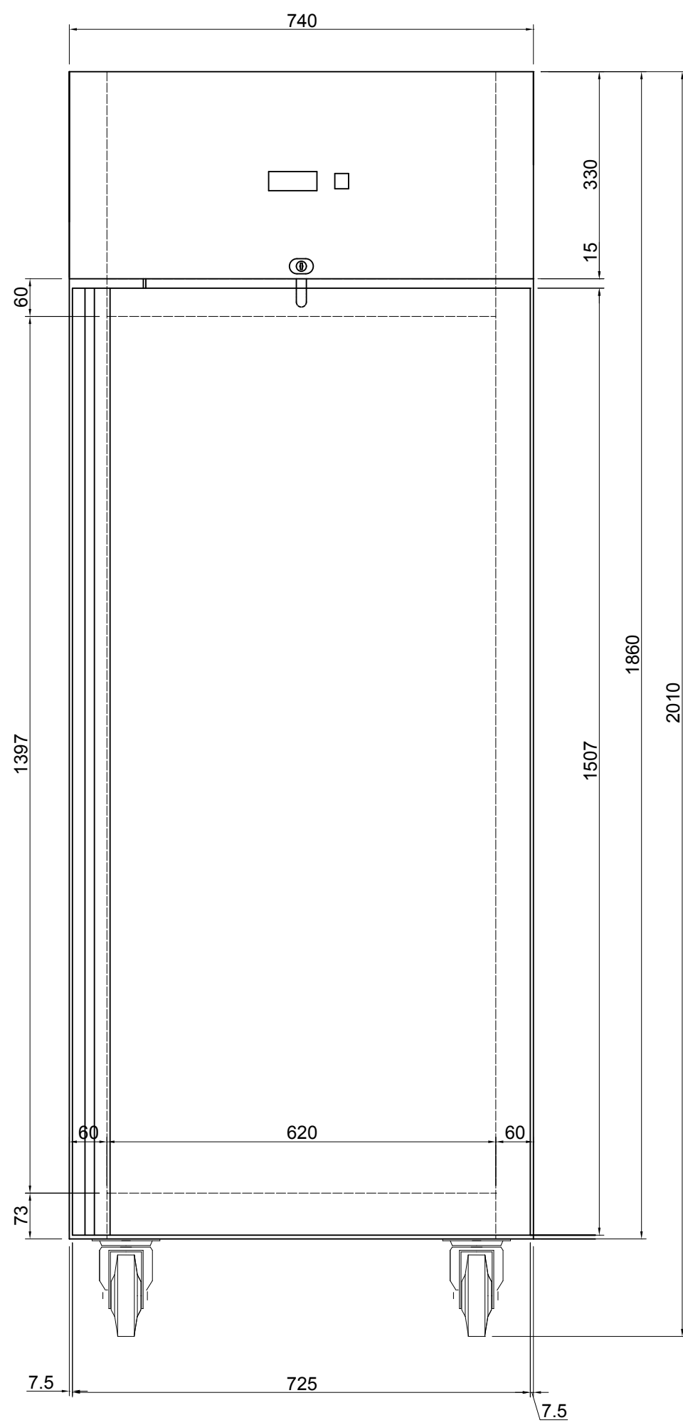
OUTSIDE SIZE OF PA800TN/BT
