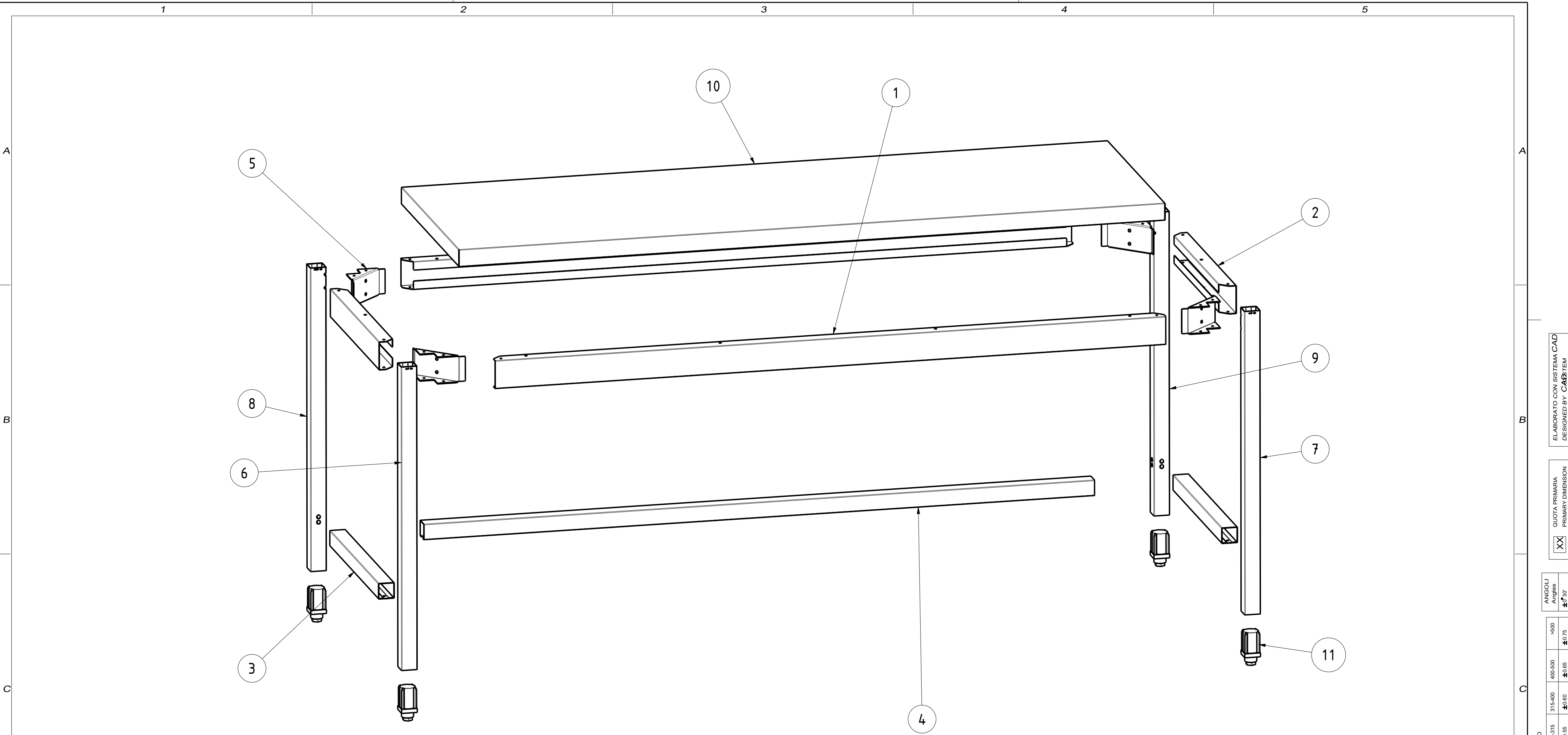
EXPLODED VIEW 3:20
