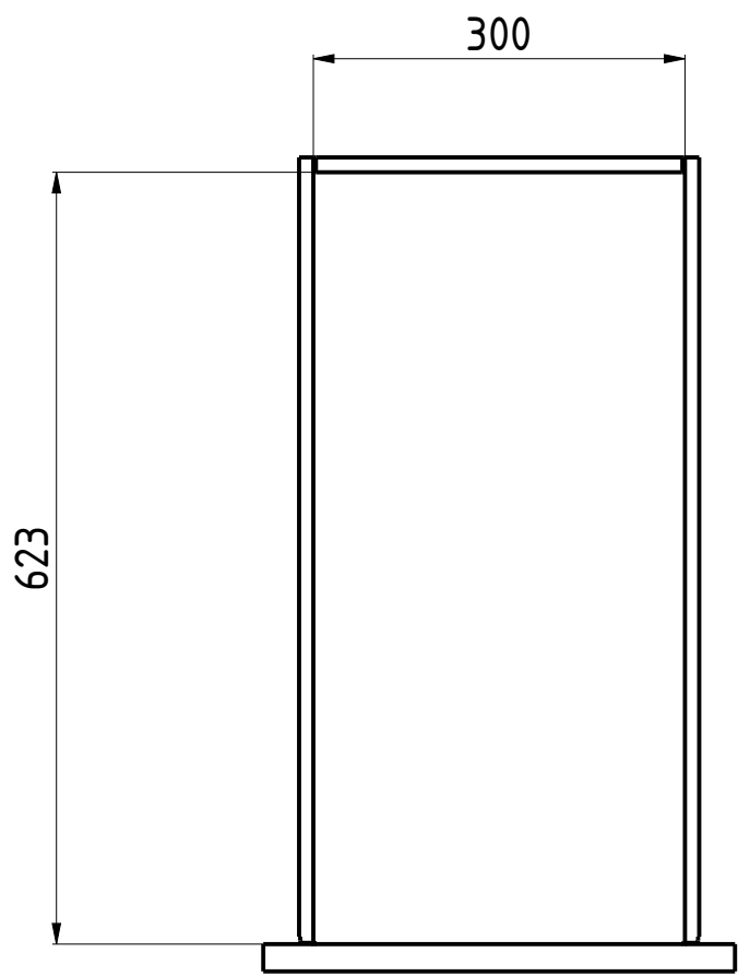
DRAWER 3:20
