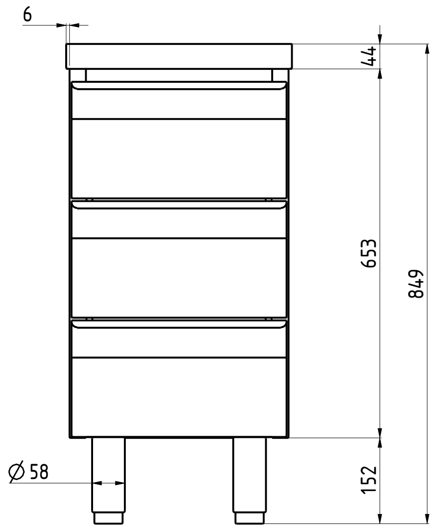
FRONT VIEW 3:20
