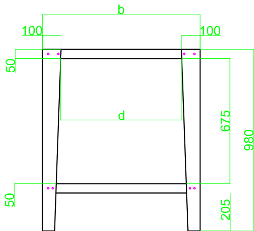
VISTA LATERALE Side view
